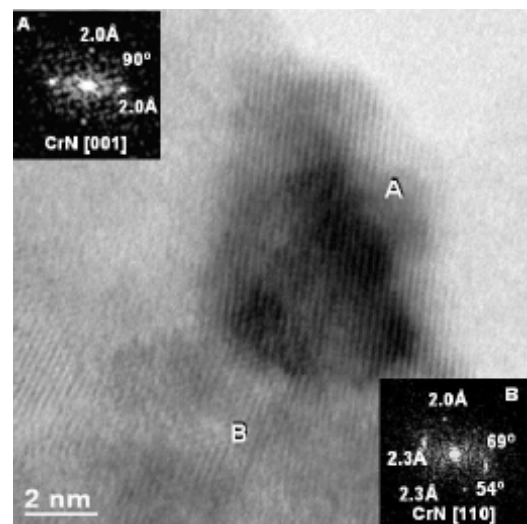
Fig 1. CrAlN sputtered nanocoating.TEM.( Fundacion INASMET)
