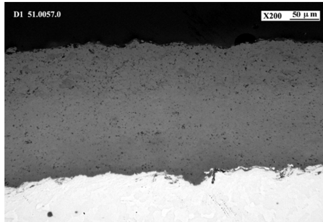
Fig 2. Yttria stabilized zirconia thermal sprayed nanocoating. SEM (Fundacion INASMET)
